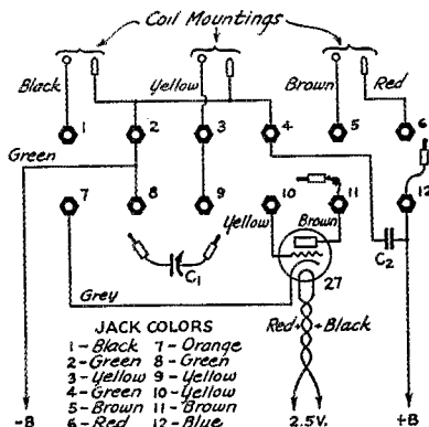
FIG. 1—CIRCUIT DIAGRAM OF THE MULTI-PURPOSE UNIT
